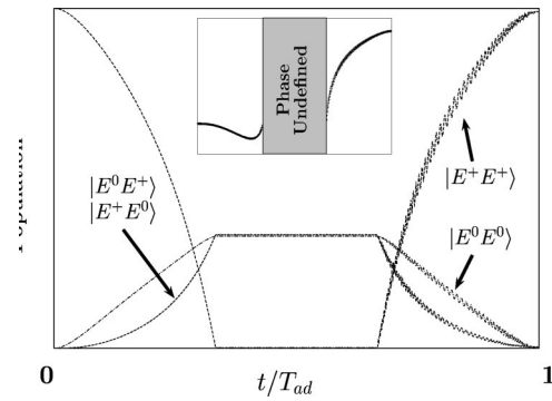
FIG. 3. Simulated control shift over the state |E^+\rangle^{\otimes 2} . The inset shows (where it is defined) the quantity \varphi^+ := \text{Arg}\langle \Psi(t) | E^+ E^+ \rangle / |\langle \Psi(t) | E^+ E^+ \rangle| . The values of the parameters are \delta = 5 meV, |\Omega_{0,+}| = \delta/5 , T_{ad} = 0.8 ns. The gate fidelity F = |\langle E^+ E^+ | \Psi(T_{ad}) \rangle|^2 = 0.9899 .
