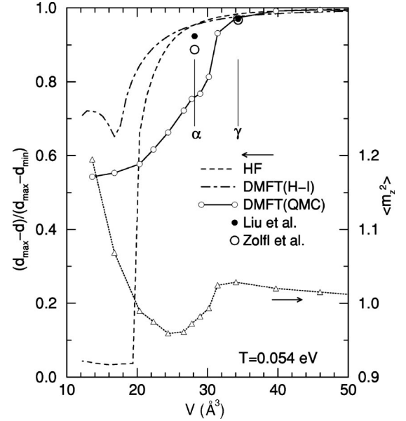
FIG. 14. Double occupation ratio (d_{\max} - d)/(d_{\max} - d_{\min}) and local magnetic moment \langle m_z^2 \rangle (triangles) as a function of volume at T = 0.054 eV. In the former case, we compare the LDA + DMFT(QMC) results with our HF and LDA + DMFT(H-I) results as well as with the LDA + DMFT(NCA) by Zöfl et al. 40 and the Anderson model calculations by Liu et al. 5 The double occupancy increases when going from \gamma - to \alpha -Ce (experimental volumes as indicated), i.e., the electrons become more itinerant or less correlated. This effect is most pronounced in our LDA + DMFT(QMC) results; however, the d ratio is still far from the uncorrelated value d = d_{\min} , i.e., \alpha -Ce is still strongly correlated.
