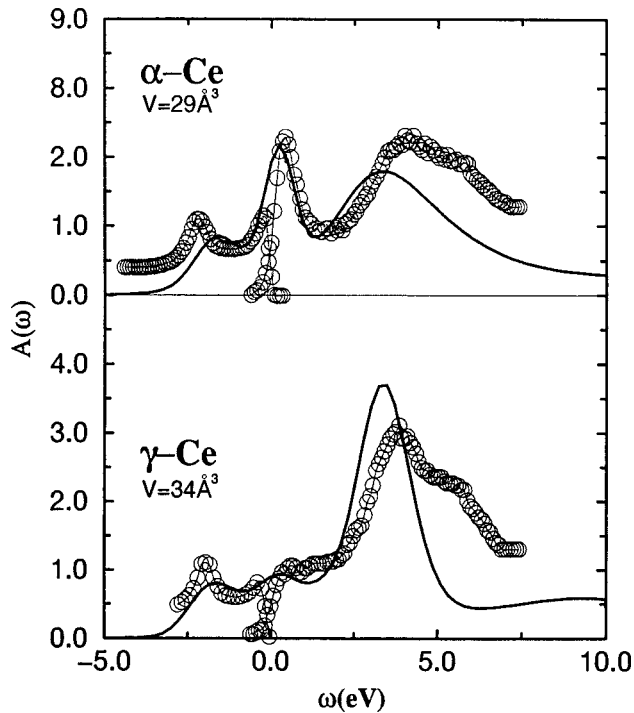
FIG. 11. Comparison of the LDA+DMFT(QMC) spectra with experiment (circles). 5 Although there are no free parameters in the calculated spectrum, the agreement is very good, in particular at the Fermi energy ( \omega=0 ). The additional structure in the upper Hubbard band which is seen in the experiment is likely due to the exchange interaction that was neglected in our calculation.
