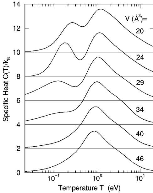
FIG. 5. Specific heat as a function of temperature for different volumes (offset as indicated). At smaller volumes, an additional low-energy peak develops, coinciding with the formation of an Abrikosov-Suhl resonance (see Fig. 8).
