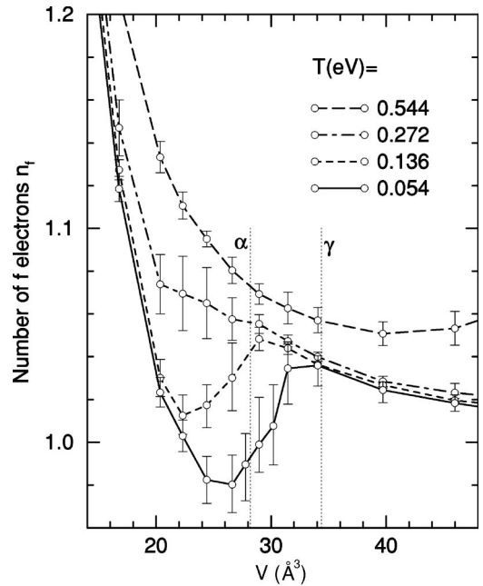
FIG. 12. Number of 4f electrons n_f vs volume at four temperatures. At low temperatures and in the vicinity of the \alpha - \gamma transition, n_f is very close to 1.
