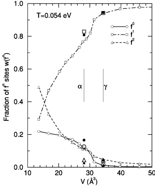
FIG. 13. Fraction of empty ( f^0 ), singly occupied ( f^1 ), and doubly occupied sites ( f^2 ) vs volume as calculated by LDA+DMFT (QMC) (open symbols with lines) at T=0.054 eV in comparison to LDA+DMFT(NCA) (large open symbols) 40 and impurity Anderson model results (filled symbols). 5 While the DMFT results agree very well for the \gamma phase, there are significant differences in the \alpha phase as discussed in the text.
