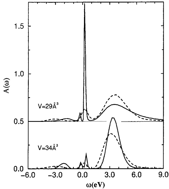
FIG. 9. 4f electron spectrum for \alpha -Ce ( V=29 \text{ \AA}^3 ) and \gamma -Ce ( V=34 \text{ \AA}^3 ) at two temperatures ( T=632 \text{ K} , solid line; T=1580 \text{ K} , dashed line). The Abrikosov-Suhl resonance of \alpha -Ce is smeared out when increasing the temperature from T=632 to 1580 \text{ K} , indicating that the Kondo temperature is in between.
