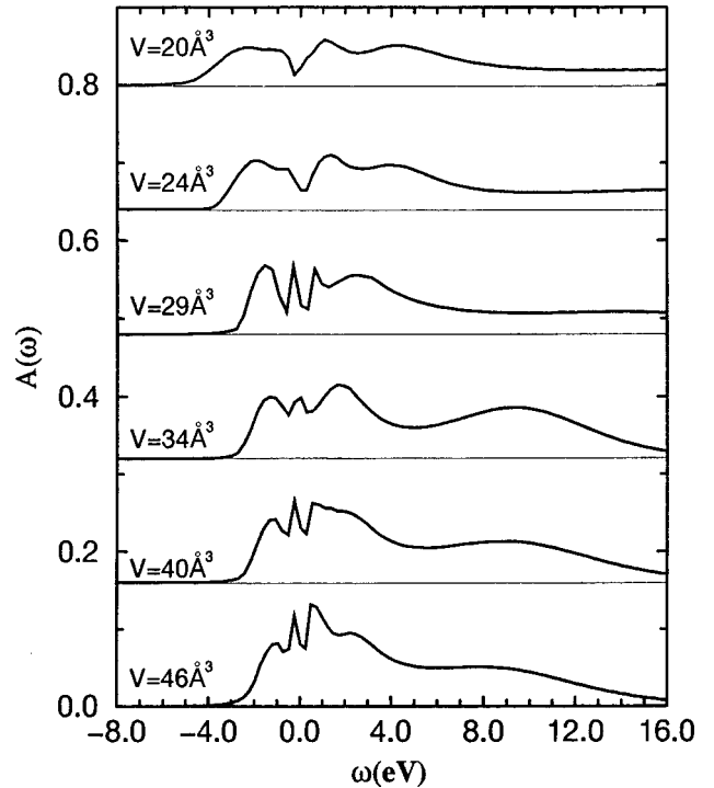
FIG. 10. Evolution of the spd electron spectrum with volume at T=632 \text{ K} ; offset as indicated. Note the wider energy window in comparison to Figs. 8 and 9. The main effect to be seen is the decrease of the bandwidth upon increasing the volume.
