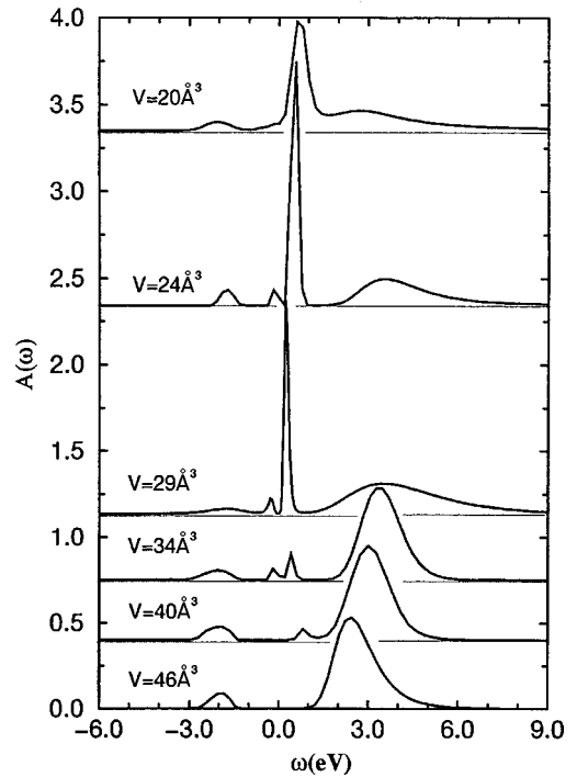
FIG. 8. Evolution of the 4f electron spectrum with volume at T=632 K; offset as indicated. When going from small to large volume, the weight of the central Abrikosov-Suhl resonance decreases and practically fades away at the \alpha - \gamma transition from V=29 to 34 \text{ \AA}^3 . The residual weight around the Fermi energy at V=34 \text{ \AA}^3 indicates a smeared out Abrikosov-Suhl resonance as is to be expected if the Kondo temperature of \gamma -Ce is below T=632 K.
