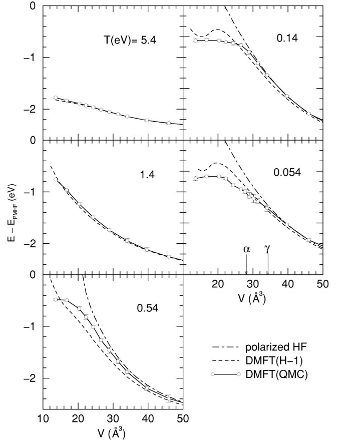
FIG. 2. Correlation energy, i.e., the difference between the LDA+DMFT and the paramagnetic HF (PMHF) energy, as a function of volume at five temperatures. At large volumes, the LDA+DMFT(QMC) energy agrees with the polarized HF and the Hubbard-I (H-I) solutions. But the LDA+DMFT(QMC) energy breaks away from the polarized HF energy for decreasing volume, leading to a region of negative curvature in the vicinity of the experimentally observed \alpha - \gamma transition (indicated by arrows) at low temperature.
