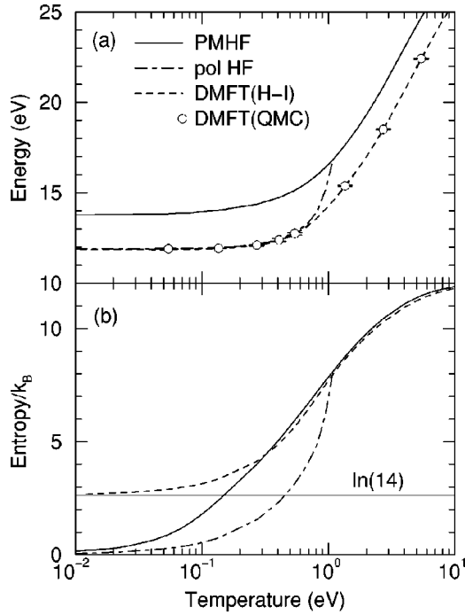
FIG. 3. Energy (upper figure) and entropy (lower figure) of the LDA+DMFT Hamiltonian Eq. (1) vs temperature at V=46 \text{ \AA}^3 . At this relatively large volume, the DMFT(QMC) and DMFT(H-I) energies agree with each other and, at lower temperatures, also with the polarized Hartree-Fock solution. However, the entropy of the latter is completely wrong since the 14-fold degeneracy of the local magnetic moment is disregarded.
