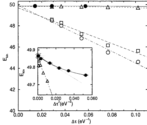
FIG. 1. Extrapolation \Delta\tau \rightarrow 0 of the kinetic energy at T = 0.54 eV and V = 16.8 \text{ \AA}^3 , using the QMC 2 (filled circles) and the QMC 1 algorithms (open circles, squares, and triangles; differences are due to whether and how Hartree-Fock results for the high-frequency tails of self-energy are included, see text). The lines show the extrapolations through the QMC data yielding E_{\text{kin}}(\Delta\tau=0) = 49.888 \pm 0.003 eV (filled circles) and 49.853 \pm 0.022 eV (open triangles), both with a mixed quadratic and cubic fit; and 49.944 \pm 0.271 eV (open circles) and 49.713 \pm 0.305 eV (open squares), both with a linear fit. The results agree within twice the above standard deviation and, thus, validate the QMC 2 algorithm. The inset shows the two upper curves (filled circles and open triangles) as a function of \Delta\tau^2 over an expanded \Delta\tau range. For the QMC 2 (filled circles) it also compares the mixed quadratic/cubic fit (solid line) with a purely quadratic fit to the data points which fulfill \Delta\tau U_f/2 \leq 0.4 (dotted line).
