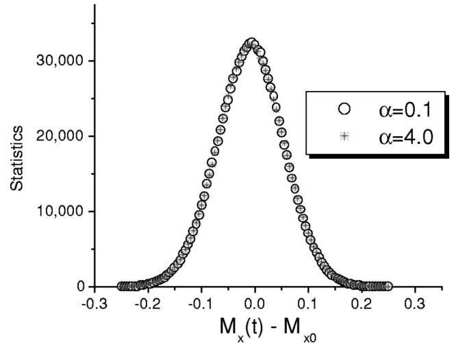
FIG. 2. Distribution of moment deviations of the x component for fixed y component, for two values of \alpha . KV/k_B T = 7.18 . Angle between the applied field H = 0.9K_z V and anisotropy axis is \pi/2 .
