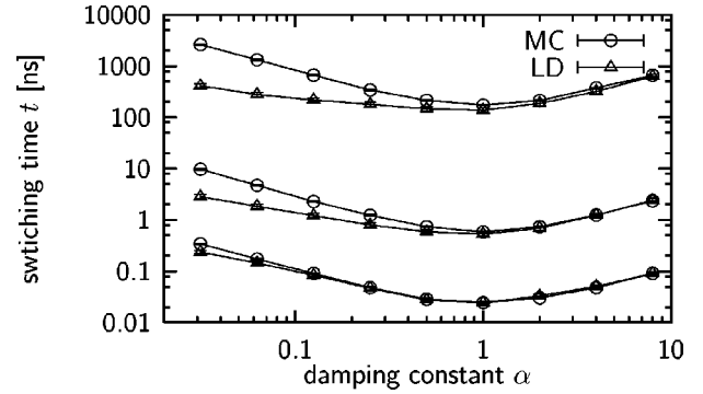
FIG. 4. Average switching time versus damping constant for a magnetic moment in a field H/2KV=0.42 applied under an angle of \pi/20 to the easy axis for different temperatures 2KV/k_B T = 72, 7.2, 2.1 (from top).
