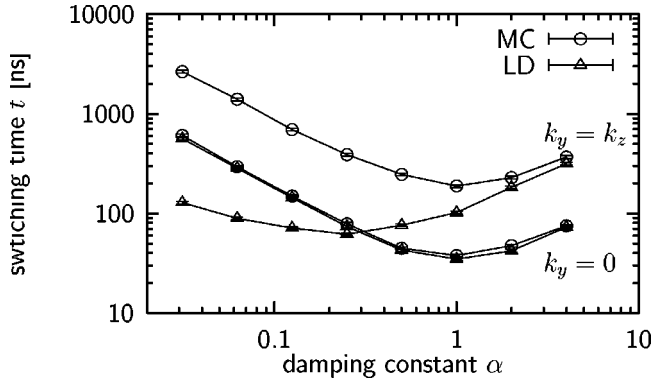
FIG. 6. Average switching time versus damping constant for a magnetic moment with an easy axis anisotropy 2K_z V/k_B T=100 and different additional hard axis anisotropies. The applied field H/2K_z V=0.9 is parallel to the easy axis.
