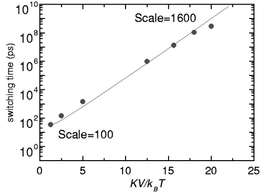
FIG. 8. Average switching time vs energy barrier calculated with TQMC compared with Aharoni's asymptote (Ref. 6) for the axially symmetric case. During the simulation the trial MC step size R=0.111 was kept constant. The corresponding quantified time step \Delta t_{\text{MC}} was increased proportionally to the barrier size \Delta t_{\text{MC}} = \text{Scale} \times \Delta t_{\text{LL}} where \Delta t_{\text{LL}}=0.01 of the precession period is the normal Landau-Lifshitz integration time step. The parameters of the simulation \alpha=0.1 , H_{\text{app}}=0.15 .
