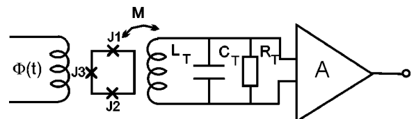
FIG. 1. Phase qubit coupled to a tank circuit.
