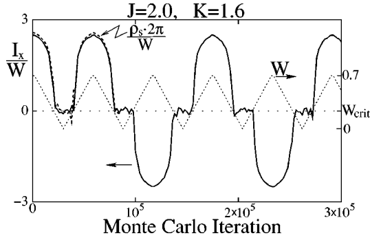
FIG. 4. Flux trapping experiment at J=2.0 and K=1.6 . The system (of size 8^3 ) is prepared with a single vortex in the annulus encircled by the L_x , deep in the SC phase ( W=0.7 ; cf. Fig. 3). The vortex is detected by measuring the circulation I_x of the superfluid current (solid line). The system is cycled between the SC and \mathcal{I}^* phases. The “sawtooth” dotted line is the Monte Carlo time variation of W drawn so that the critical W_{\text{crit}} coincides with the zero of I_x . For a trapped vortex, the magnitude of I_x is set by the superfluid stiffness and is expected to be \approx \rho_s 2\pi . The latter is shown with a dashed line for the first two cycles; the fact that the two quantities coincide indicates that the vortex remains trapped across the transition.
