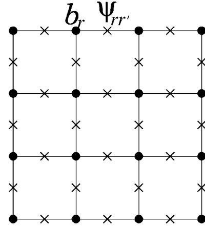
FIG. 1. Face-centered square lattice on which our model Eq. (1) is defined.
