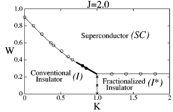
FIG. 3. Phase diagram of the classical model Eq. (10) at fixed J=2.0 . We label the phases using the language of the original quantum model Eq. (1): Superconductor SC is an XY ordered phase, while insulators \mathcal{I} and \mathcal{I}^* are two magnetically disordered but topologically distinct phases of the classical problem.
