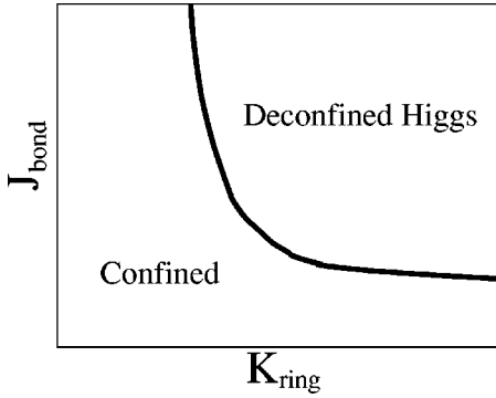
FIG. 2. Phase diagram of the (2+1)-dimensional compact QED coupled to a charge 2 scalar.
