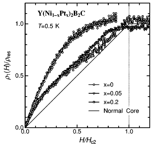
FIG. 3. Real part of the complex resistivity as a function of the magnetic field. Vertical and horizontal axes are normalized by \rho_{res} and H_{c2} , respectively.
