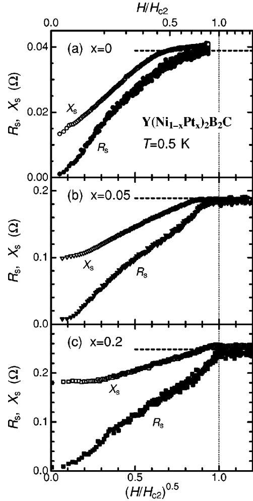
FIG. 1. Magnetic field dependence of the surface impedance of \text{Y}(\text{Ni}_{1-x}\text{Pt}_x)_2\text{B}_2\text{C} plotted as a function of \sqrt{H/H_{c2}} . Horizontal dashed lines denote the normal state values just above T_c .
