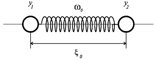
FIG. 3. Schematic picture explaining notations of Eqs. (23) and (24).
