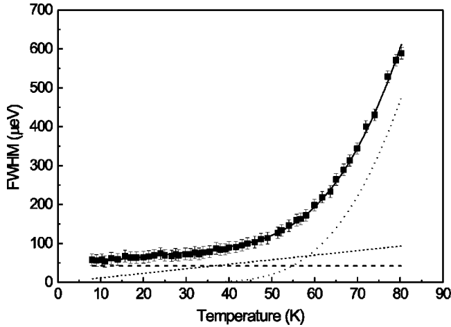
FIG. 3. Temperature dependence of the homogeneous linewidth of one narrow line. The experimental data (squares) were fitted by Eq. (1) (solid line). The contributions to the linewidth from acoustic-phonon scattering and LO-phonon scattering are also shown (short-dashed and dotted lines, respectively). The dashed line represents the low-temperature limit of the linewidth.
