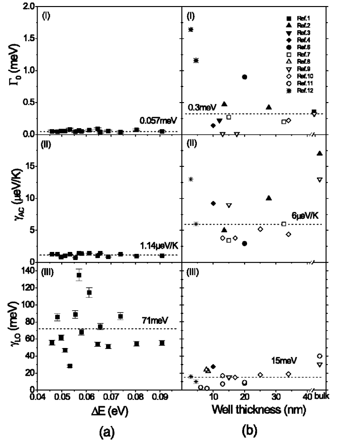
FIG. 4. (a) Low-temperature limits of linewidth (I), exciton-acoustic-phonon interaction coefficients (II) and exciton-LO-phonon interaction coefficients (III) gained by fitting the measured \Gamma \sim T relations (see Fig. 3). The error bars show the uncertainty of the fitting due to a limited temperature range, as discussed in the text. The dashed lines represent the average values. (b) The corresponding available values for quasi-two-dimensional excitons in GaAs quantum wells and excitons in GaAs bulk and superlattices. References for all data points are listed in (b)I.
