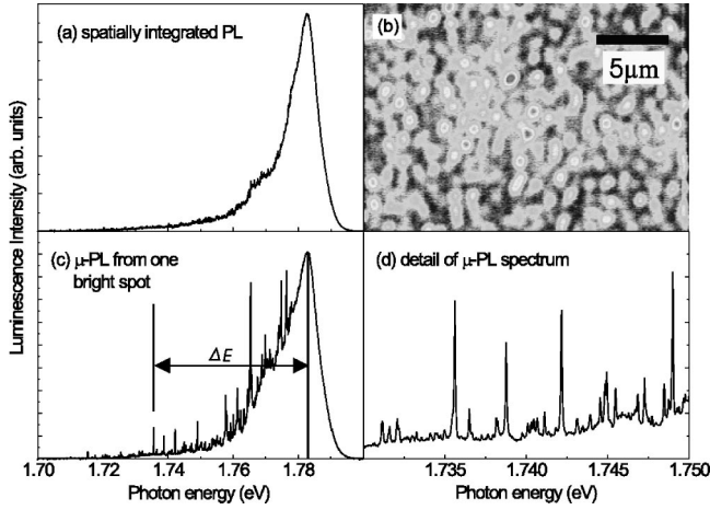
FIG. 1. Luminescence of GaAs/AlAs superlattices at 20 K under excitation of He-Ne laser with an excitation intensity of about 1 \text{ W/cm}^2 . (a) Spatially integrated PL spectrum. (b) Intensity maps. (c) The \mu -PL spectrum of one of the bright spots. (d) Details of (c). The intensity maps are recorded by blocking the scattered light from the laser, and spectrally integrating the luminescence from 1.7 to 1.8 eV.
