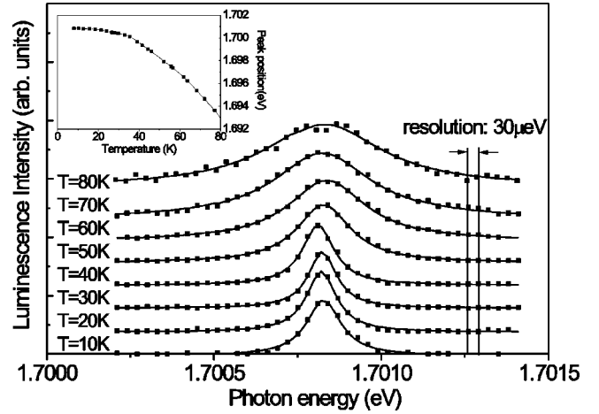
FIG. 2. An example of the measured narrow lines (squares) and the corresponding Lorentzian fit (solid line). The peak positions have been shifted for better illumination. For the actual positions under different temperatures, see the inset.
