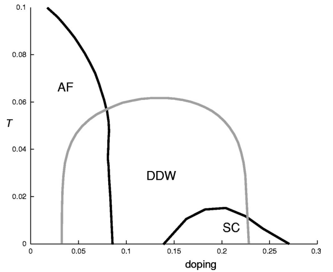
FIG. 2. Phase diagram for t=0.5 eV, t'=0 , t_{\perp}=0.1 eV, U \approx 0.042 eV, V \approx 1.7 \times 10^{-4} eV, and t_c \approx 1.5 \times 10^{-3} eV. ( g_{\text{AF}}=0.084 eV, g_{\text{DDW}}=0.038 eV, and g_{\text{DSC}}=0.017 eV.)
