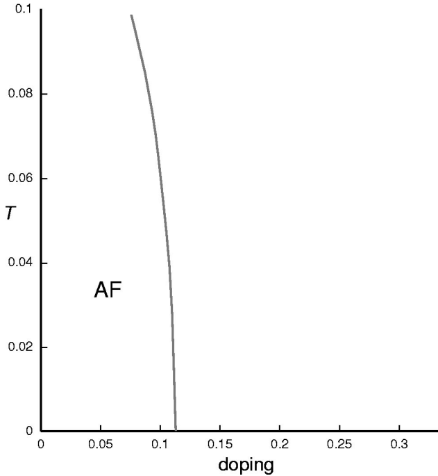
FIG. 3. Phase diagram for t=0.5 eV, t'=-0.025 eV, t_{\perp}=0.05 eV, U=0.05 eV, V=0 eV, and t_c \approx 3.3 \times 10^{-4} eV. ( g_{AF}=0.1 eV, g_{DDW}=0.008 eV, and g_{DSC}=0.004 eV.)
