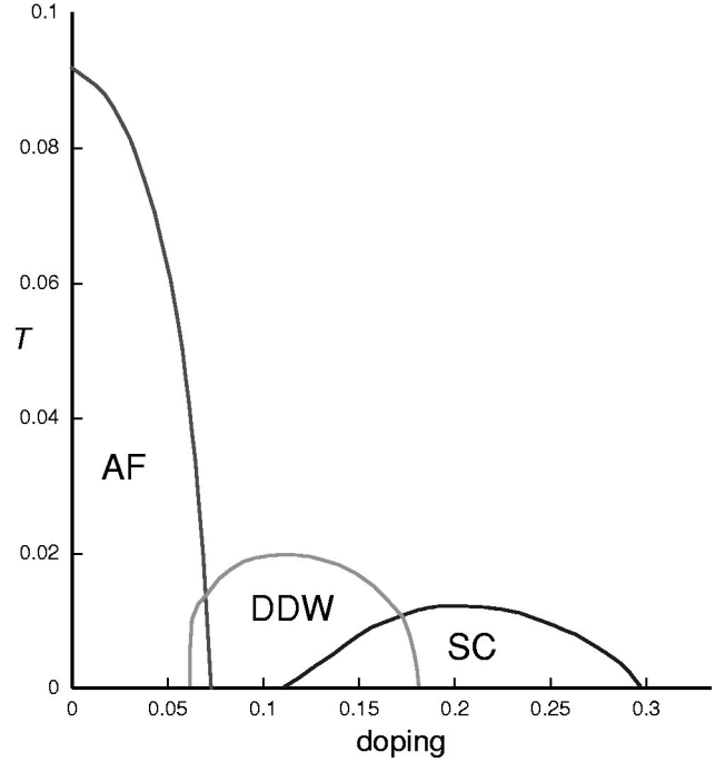
FIG. 1. Phase diagram for t=0.5 eV, t'=-0.025 eV, t_{\perp}=0.05 eV, U \approx 0.03 eV, V=0 eV, and t_c \approx 0.8 \times 10^{-3} eV. ( g_{\text{AF}}=0.06 eV, g_{\text{DDW}}=0.02 eV, and g_{\text{DSC}}=0.01 eV.) T is given in eV.
