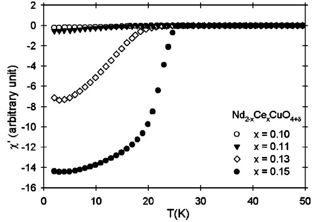
FIG. 1. Temperature dependence of the ac magnetic susceptibility \chi' (real part) for the NCCO powder samples used in the neutron measurements. The background was subtracted using \chi' for x=0.09 , which shows a Curie-Weiss-like behavior down to the lowest temperature measured. The diamagnetic signal first appears for x \geq 0.11 .
