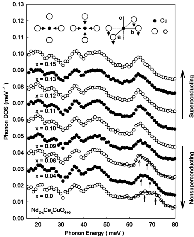
FIG. 2. The GDOS of NCCO as a function of x at T=30 K. Each GDOS is displaced along the vertical axis for clarity, and the solid lines are Gaussian fits discussed in the text. The nonsuperconducting-superconducting transition as a function of x is schematically shown on the right. The insets show the polarizations of the oxygen half-breathing (left), breathing (middle), and out-of-plane (right) vibrational modes.
