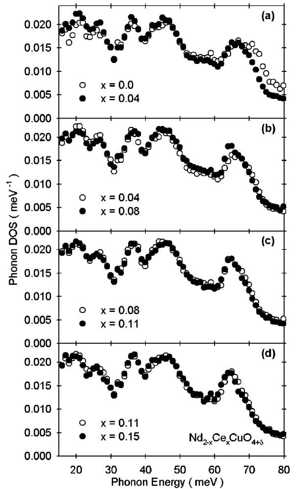
FIG. 3. Comparison of the GDOS of NCCO as a function of electron-doping, x . (a) The GDOS of NCCO for x=0.0 and 0.04 , (b) x=0.04 and 0.08 , (c) x=0.08 and 0.11 , and (d) x=0.11 and 0.15 . The finite value of the GDOS above the phonon cut off energy at 80 meV is due to the uncorrected multiphonon contributions; we were unable to make more accurate multiphonon corrections because of the difficulty in eliminating the magnetic contributions to the total scattering. However, a better correction for multiphonon contributions should have no significant influence on the major conclusions drawn from the data.
