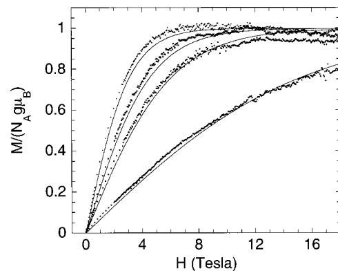
FIG. 5. Comparison between experiment and theory (including diamagnetic contribution) for the magnetization M of compound 1 for static magnetic fields H up to 18 T for T = 2, 3, 4, 10 K. As discussed in the text, for the choices of J , \Delta , and g made in Sec. II C 1, the paramagnetic behavior in this regime of temperatures and fields is accurately described in terms of noninteracting triangles each pictured as a single spin-1/2 particle.
