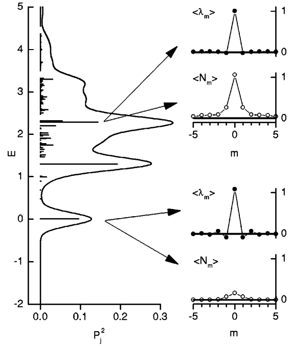
FIG. 1. Illustration of the eigenstates and their properties for a numerical solution of the Holstein model (1) with parameters J = 0.5 and g = 1 at total momentum k = 0 . In the left panel, the optically active eigenstates are shown at a vertical energy axis. The sticks indicate the spectral weight P_j^2 of each state according to Eq. (17). For a visualization of the resulting spectrum, the stick spectrum is convolved with a Gaussian (standard deviation \sigma = 0.15 ) and the broadened spectrum is scaled for easy superposition [here, area \int f(E) dE = 0.5 ]. In the right panels, the occupation number clouds \langle \hat{N}_m \rangle and displacement clouds \langle \hat{\lambda}_m \rangle are shown for two particular eigenstates [see comments to Eqs. (20) and (21)].
