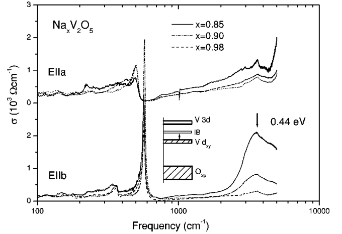
FIG. 4. Optical conductivity of \alpha' - \text{Na}_x\text{V}_2\text{O}_5 obtained from the Kramers-Kronig analysis of the reflectivity spectra in E\parallel a (top panel) polarizations, and E\parallel b (lower panel). Inset: Schematic representation of the \text{V}3d_{x,y}\text{-IB} transitions.
