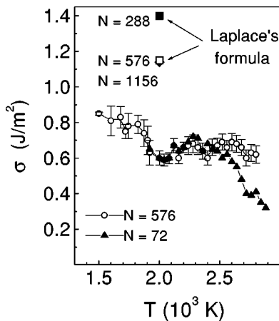
FIG. 13. Surface tension as a function of the temperature for the clusters with N=72 atoms (triangulars) and N=576 atoms (open circles). The three points above denote the surface tension from Laplace's formula for the clusters with 288 atoms (squares), 576 atom (diamonds), and 1156 atoms (open squares).
