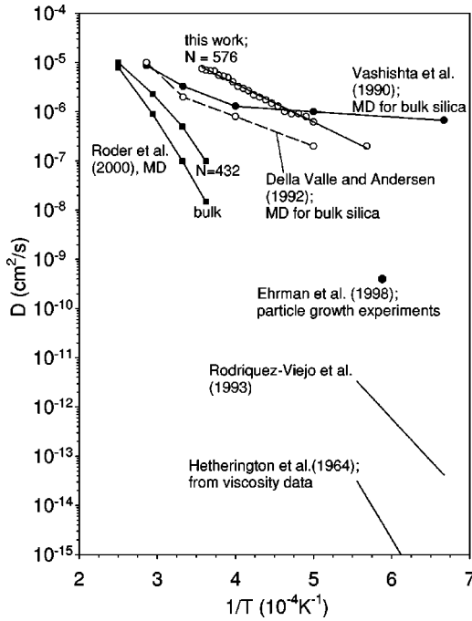
FIG. 10. Diffusion coefficient for silicon atoms from the calculations and experiments.
