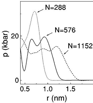
FIG. 12. The smoothed radial pressure distribution for clusters with N=288 atoms (dotted line), N=576 atoms (solid line) and N=1152 atoms (dashed lined line) at T=2000 K.
