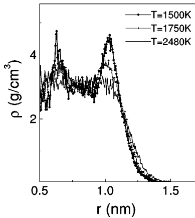
FIG. 2. Radial density distribution for the cluster with 576 atoms at different temperatures.
