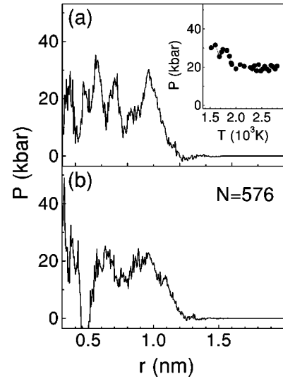
FIG. 11. Radial pressure distribution for the N=576 atom cluster at T=1760 K (a), and T=2000 K (b). Surface pressure as a function of temperature is shown in the inset.
