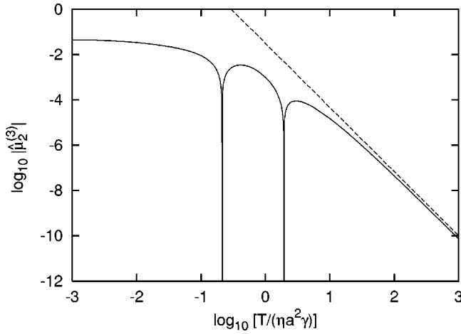
FIG. 4. Double logarithmic plot of the rectified velocity [the dimensionless quantity \hat{\mu}_{2,\text{ad}}^{(3)} given in Eq. (76)] vs temperature in the adiabatic limit for potential (72) in the underdamped case \alpha = \frac{1}{2} (bold line). The dashed line is a guide to the eye, representing the behavior \propto T^{-17/6} of the high-temperature limit.
