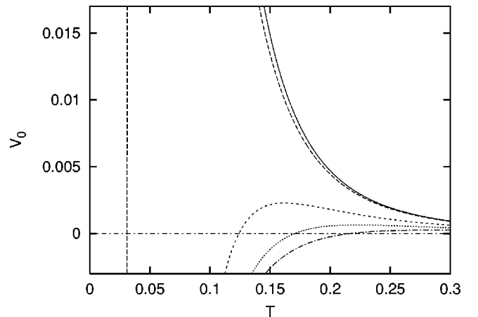
FIG. 2. V_0(T) for \omega = 0.01 (bold line), \omega = 1 (long dashes), \omega = 4 (short dashes), \omega = 5.5 (dotted line), and \omega = 7 (dash-dotted line) for comparison with Fig. 1(a) in Ref. 17. The vertical line represents the vicinity of the current reversal for \omega = 1 .
