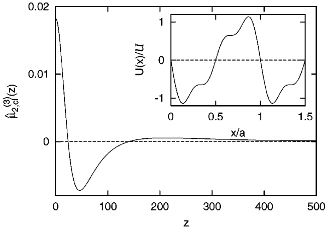
FIG. 3. Scaling function \hat{\mu}_{2,cl}^{(3)}(z) for potential (73) shown in the inset.
