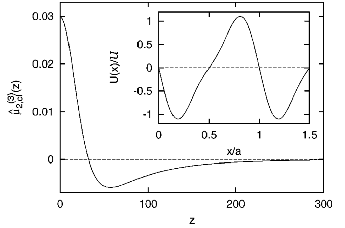
FIG. 1. Scaling function \hat{\mu}_{2,\text{cl}}^{(3)}(z) for potential (72) shown in the inset.
