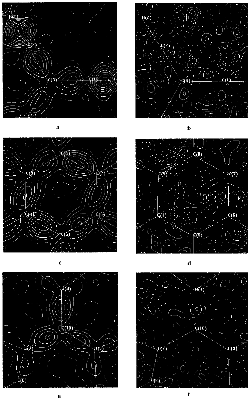
FIG. 3. Dynamic and residual maps for the (a/b) nitrile, (c/d) phenyl, (e/f) substitution point of the -\text{C}(\text{NEt})_2 group in DED-TCNQ out to \sin \theta/\lambda = 0.7 \text{ \AA}^{-1} and with contour levels of 0.1 e/\text{\AA} . (Solid lines are positive, dashed lines are negative, and dotted lines are zero.)
