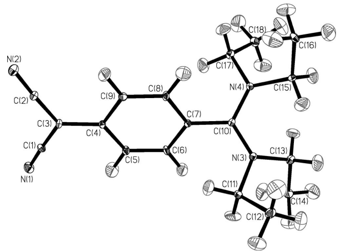
FIG. 2. A 50% probability thermal ellipsoid plot of the 20 K neutron structure of DED-TCNQ.
