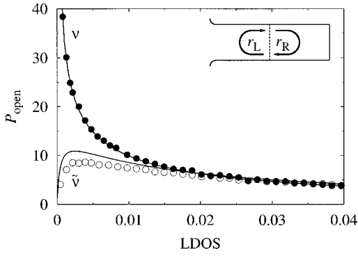
FIG. 1. Distributions of the microscopic local density of states (LDOS) \nu and the mesoscopic LDOS \tilde{\nu} for the open wire at a distance L=2l from the opening. [Both are measured in units of their mean \nu_0=(\pi\nu)^{-1} .] Solid curves are given by Eqs. (10) and (13). The data points result from a numerical simulation for a wire of length 10l with no adjustable parameter. The inset shows the geometry of the open wire (not to scale).
