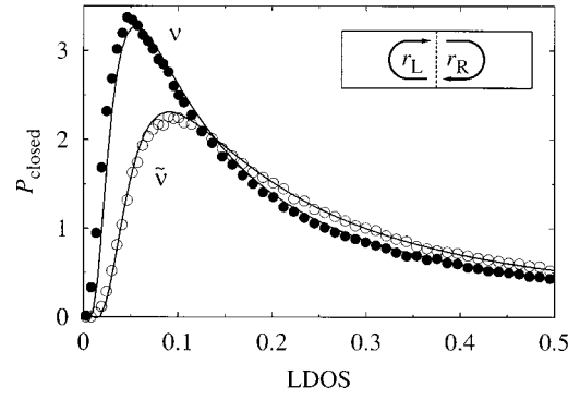
FIG. 2. Same as in Fig. 1 but for the closed wire with dimensionless absorption rate \omega=1/6 . Solid curves are given by Eqs. (17) and (19). The data points result from a numerical simulation for a wire of length 55l , with the LDOS computed halfway in the wire.
