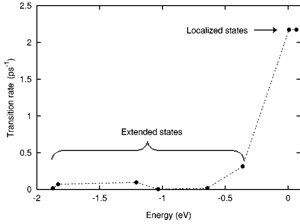
FIG. 4. Transition rates for the states within 2 eV below the Fermi level when the external field is 0.8 V/Å. The localized states are partially filled because of the Gaussian broadening of 0.1 eV used in the density of states.
