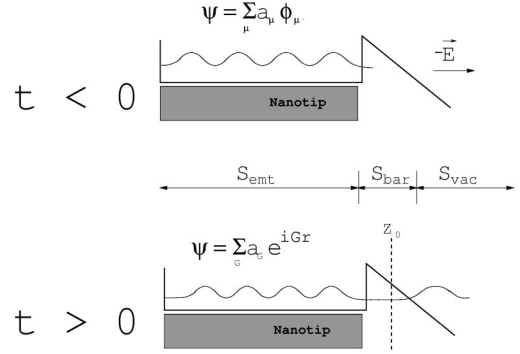
FIG. 1. Computational scheme for evaluating the transition rate of an electronic state. The wave function is described with the localized basis ( \phi_\mu ) before the transition ( t \leq 0 ). For t > 0 , the basis is switched to plane waves ( e^{iGr} ) and the transition occurs. z_0 is the boundary used in evaluating the amount of the electron tunneling. S_{\text{emt}} , S_{\text{bar}} , and S_{\text{vac}} are the emitter, barrier, and vacuum regions, respectively.
