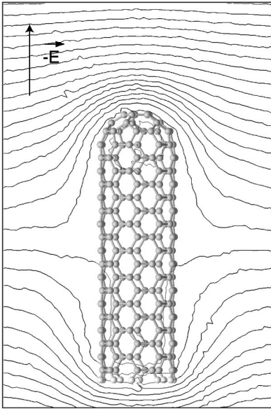
FIG. 2. Equipotential lines of the model system when the external field is 0.8 \text{ V/\AA} . Successive lines are separated by 1 \text{ V} .
