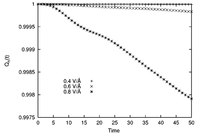
FIG. 3. Change of Q_n (the charge remaining in the nanotube) for a localized state as a function of elapsed time. The data are plotted for three different external fields ( 0.4 , 0.6 , and 0.8 \text{ V/\AA} ).
