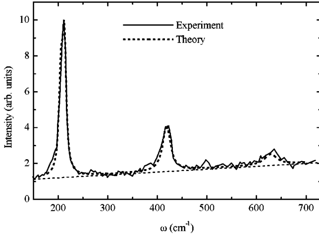
FIG. 1. Multiphonon Raman-scattering spectrum for the ensemble of CdSe nanocrystals with \langle R \rangle = 2 nm compared with the experimental data of Ref. 6. The thin dashed line is the luminescence background. The following parameter values are used: \varepsilon_1(\infty) = 6.23 , \varepsilon_1(0) = 9.56 (Ref. 51), m_e = 0.11m_0 , E_g = 1.9 eV (Ref. 52), \gamma_1 = 2.04 , \gamma_2 = 0.58 (Ref. 53), and \varepsilon_2 = 2.25 (Ref. 6).
