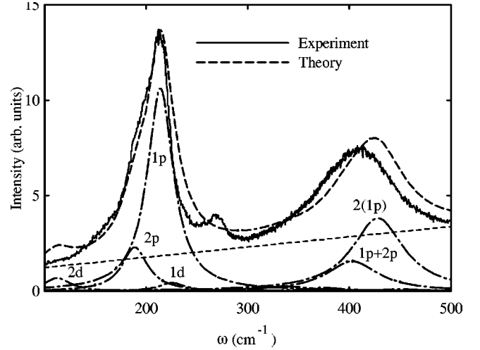
FIG. 2. Calculated Raman-scattering spectrum (the heavy dashed curve) for the ensemble of PbS nanocrystals with \langle R \rangle = 1.5 nm. The experimental spectrum of Ref. 8 is shown by the solid line. The following parameter values are used: E_g = 0.307 eV (Ref. 54); \varepsilon_1(\infty) = 18.5 , \varepsilon_1(0) = 190 (Ref. 55).
