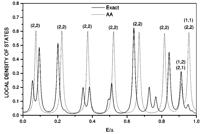
FIG. 4. Plot of the LDOS against E/\Delta for x = 1000 Bohr, L_t = 12.5676 Bohr, L = 4000 Bohr, and \Delta = 0.0001 Ry.
