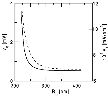
FIG. 5. Coefficients v_0 (solid curve, left scale) and v_1 (dashed curve, right scale) of adjusted polynomial [Eq. (14)] as functions of outer radius R_b of surface \Sigma , on which we put the boundary conditions for the Poisson equation.
