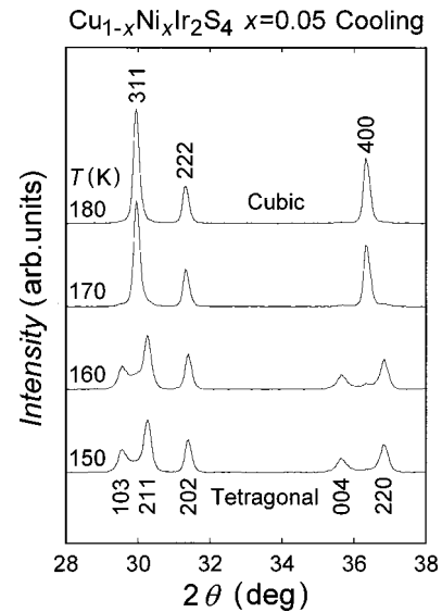
FIG. 6. Temperature dependence of the powder x-ray diffraction pattern for x=0.05 upon cooling. At 150 K, the only tetragonal phase is detected.
