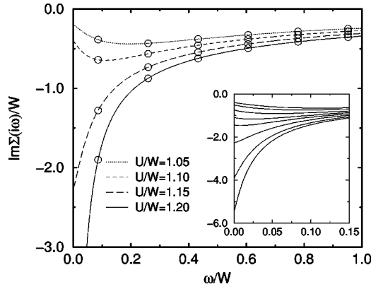
FIG. 6. Imaginary part of the self-energy, \text{Im} \Sigma , on the imaginary frequency axis for the same parameters as in Figs. 3 and 5. The values of \text{Im} \Sigma for the Matsubara frequencies are indicated by the circles. The inset focuses on the change of sign of the slope in \text{Im} \Sigma(i\omega) for values of U = 1.1W up to U = 1.17W (from top to bottom).
