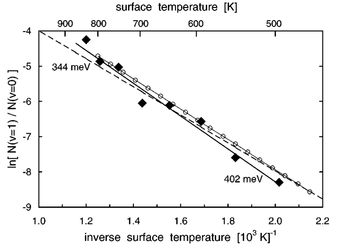
FIG. 6. Arrhenius plot of the relative population in the state v''=1 as a function of the inverse surface temperature T_S^{-1} . The straight line is a least-squares fit to the data, the dashed line a fit with a forced equilibrium population at T_S=\infty , and the open symbols denote theoretical results.
