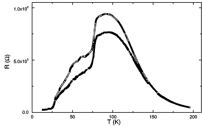
FIG. 13. Resistance versus temperature measured under illumination with applied magnetic field of B=0.48 T (solid squares) and without (open circles) for sample 1498.
