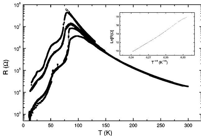
FIG. 8. Resistance versus temperature measured in darkness (open dots) and under illumination (solid dots) with different optical power for the least oxygenated sample (No. 1611).
