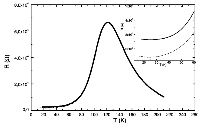
FIG. 3. Resistance versus temperature of a slightly oxygen deficient \text{La}_{2/3}\text{Sr}_{1/3}\text{MnO}_{3-\delta} thin film. (Sample 1504) in darkness (solid line) and after illumination (dashed line). The inset shows behavior at the low temperature on a larger scale.
