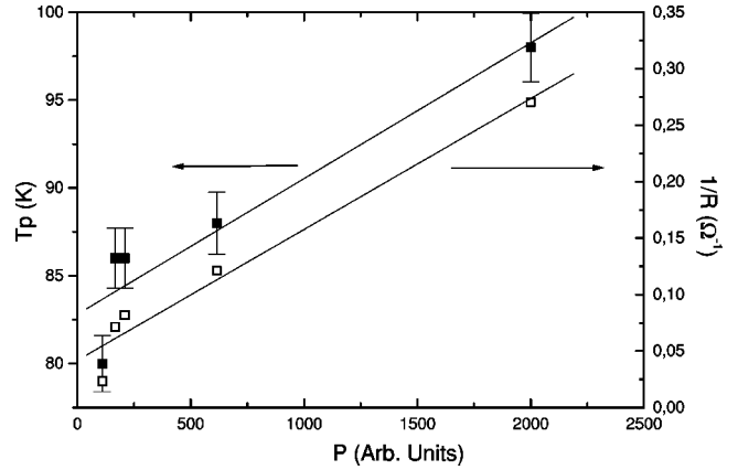
FIG. 9. Linear dependence of T_p and the corresponding value R^{-1} versus optical power.
