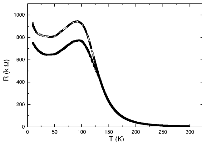
FIG. 12. Resistance versus temperature measured in darkness with an applied magnetic field of B=0.48 T (solid squares) and without (open circles) for sample 1498.
