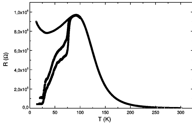
FIG. 11. Resistance versus temperature measured in darkness (open dots) and under illumination (solid dots) for two optical powers for the intermediate oxygen deficient sample (No. 1498).
