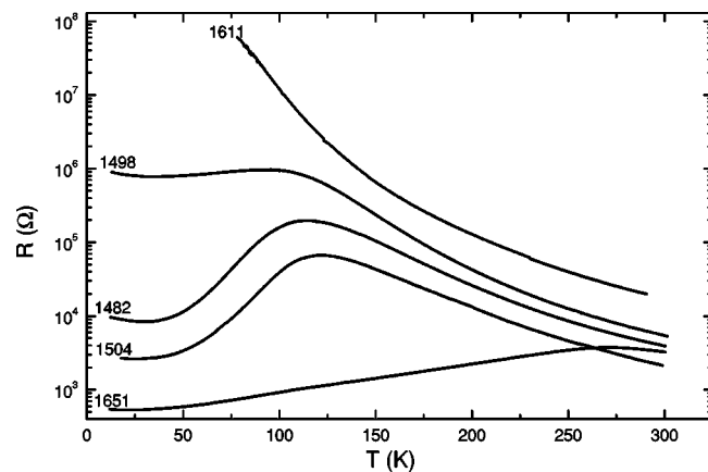
FIG. 1. Resistance versus temperature in darkness for different oxygen content \text{La}_{2/3}\text{Sr}_{1/3}\text{MnO}_{3-\delta} thin films.
