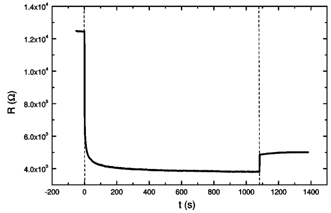
FIG. 6. Resistance versus illumination time for the sample 1482 showing persistent photoconductivity. T = 10 K.
