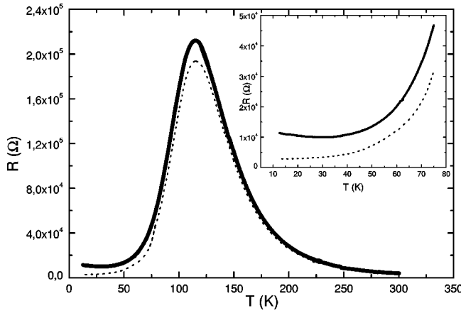
FIG. 4. Resistance versus temperature of a slightly oxygen deficient \text{La}_{2/3}\text{Sr}_{1/3}\text{Mn}_{3-\delta} thin film. (Sample 1482) in the darkness (solid line) and after illumination (dashed line). The inset shows the low-temperature behavior on an expanded scale.
