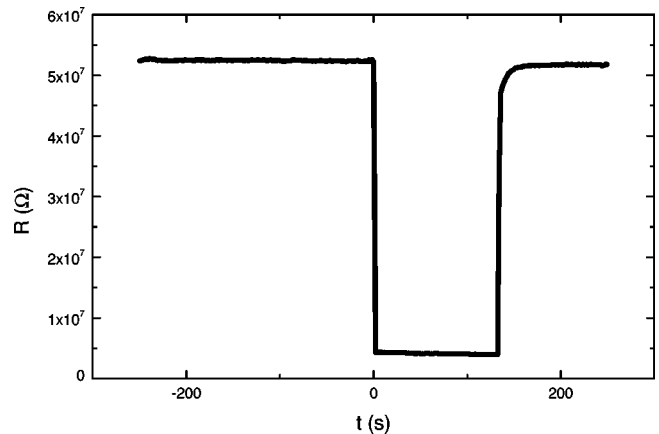
FIG. 10. Time dependence of the resistance of sample 1611 after illumination at t=0 and ceasing illumination at t=130 s.
