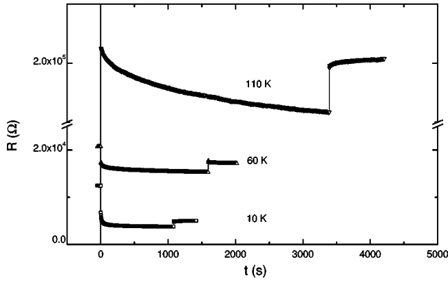
FIG. 7. Resistance versus time (sample 1482) with the same optical power at different temperatures (illumination times: 0–1080 s at 10 K, 0–1600 s at 60 K, and 0–3400 s at 110 K).
