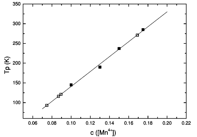
FIG. 2. T_p versus \text{Mn}^{4+} concentration. Dark squares from Ref. 16. Open squares: our measurements.
