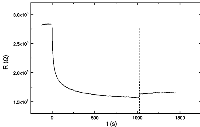
FIG. 5. Resistance versus illumination time for the sample 1504 showing persistent photoconductivity. The small increase at 1020s may be due to a heating effect as the light is turned off. T = 10 K.
