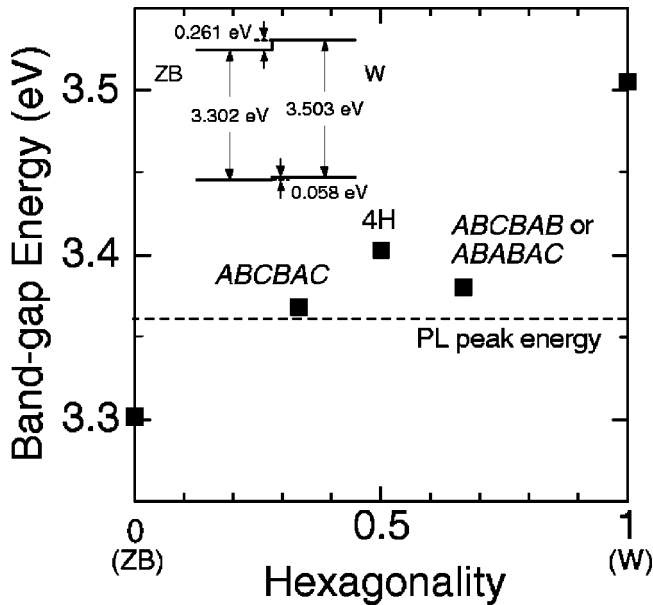
FIG. 8. Dependence of band-gap energies of several polytypes on hexagonality calculated by the simple Kronig-Penney model. The hexagonality refers to the proportion of W stacking. The dotted line indicates the PL peak position.
