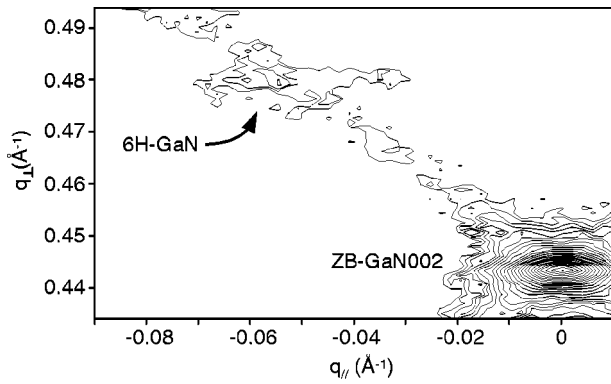
FIG. 3. The x-ray RSM of the area indicated by the rectangle in Fig. 3(a). Isointensity contour levels at 2^{n/3} ( n=0,1,2,3, \dots ) cps. The q_{\parallel} axis is parallel to the [110] direction, and the q_{\perp} axis is parallel to the [001] direction.
