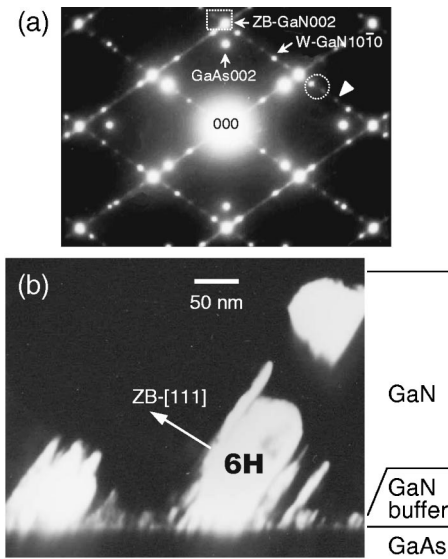
FIG. 1. (a) ED pattern and (b) TEM dark-field image of GaN grown on GaAs(001). The (\bar{1}10) cross section was observed. The arrowhead in (a) shows one of the diffraction spots from six-bilayer periodic structures. Also in (a), the circle indicates the size of the objective aperture, inside which are the diffraction spots used to generate the dark-field image of (b). The rectangle in (a) is used with Fig. 3.
