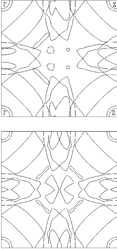
FIG. 5. Basal plane (top) and midplane ( k_z shifted by 1/4 , bottom) Fermi surfaces of \text{Sr}_3\text{Ru}_2\text{O}_7 in the experimental orthorhombic structure. Note that the zone is rotated 45^\circ with respect to the tetragonal and folded.
