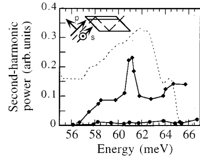
FIG. 2. Second-harmonic power as a function of the pump energy. Diamonds: n -doped quantum dot sample; dots: undoped GaAs reference sample. The dashed line shows the absorption along the [110] direction. The inset shows the waveguide geometry. The pump beam is p polarized. The lower amplitude for the GaAs reference sample is attributed to a difference in the injection and collection efficiencies.
