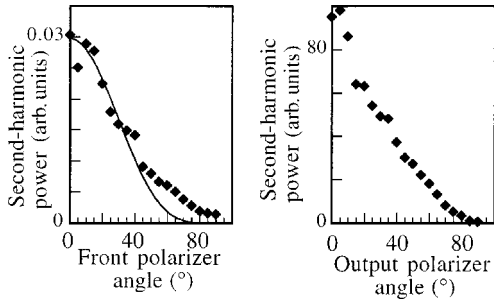
FIG. 3. Second-harmonic power as a function of the polarization angle of the incident excitation beam. 0^\circ ( 90^\circ ) corresponds to a p ( s ) polarized excitation. In p polarization, part of the electric field is along the [110] direction. In s polarization, the electric field is along the [-110] direction. The pump energy is 61 meV. The figure on the right hand side shows the second-harmonic power as a function of the output polarizer angle. The pump at 61 meV was set in p polarization.
