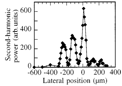
FIG. 4. Second-harmonic power of bulk GaAs as a function of the lateral position of the sample. The maxima correspond to the achievement of phase matching. The distance between two maxima corresponds to twice the coherence length.
