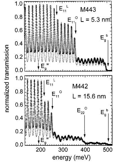
FIG. 3. Infrared optical transmission spectra measured at 5 K, for two PbTe/Pb 1-x Eu x Te MQW samples, with well width L = 5.3 and 15.6 nm. The solid lines are the results of the simulation, and the circles correspond to the measured data. The arrows indicate the main optical transitions ( E_{11}^L , E_{11}^O , and E_{22}^O ), obtained from the best-fit procedure, together with the PbTe well ( E_g^w ) and Pb 1-x Eu x Te barrier ( E_g^b ) band gaps.
