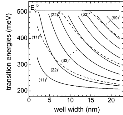
FIG. 4. Optical transition energies for \text{PbTe}/\text{Pb}_{0.93}\text{Eu}_{0.07}\text{Te} QW's (at 5 K), as a function of well width, calculated in the envelope-function approximation and the perfect square QW model. The solid (dashed) lines correspond to the energy of the longitudinal (oblique) transitions in an increasing order of subband indices. The straight line represents the top of the barrier ( E_g^b ).
