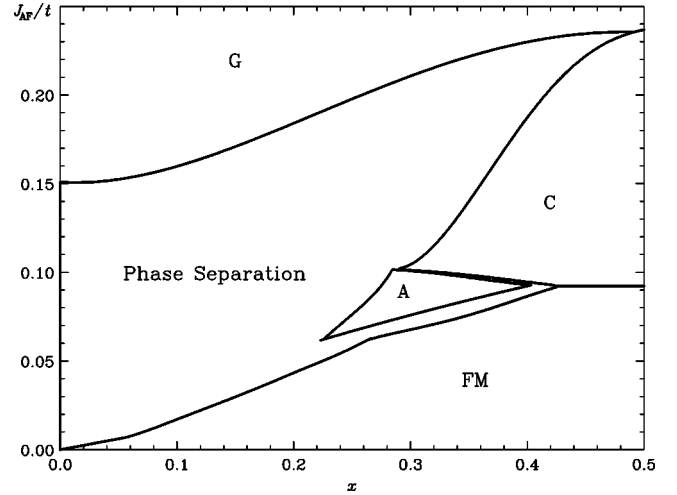
FIG. 1. Calculated phase diagram at T=0 . The A -AFM phase has ferromagnetic alignment within planes, and antiferromagnetic alignment between parallel planes. The C -AFM phase has ferromagnetic alignment along chains, and antiferromagnetic alignment between neighboring chains.
