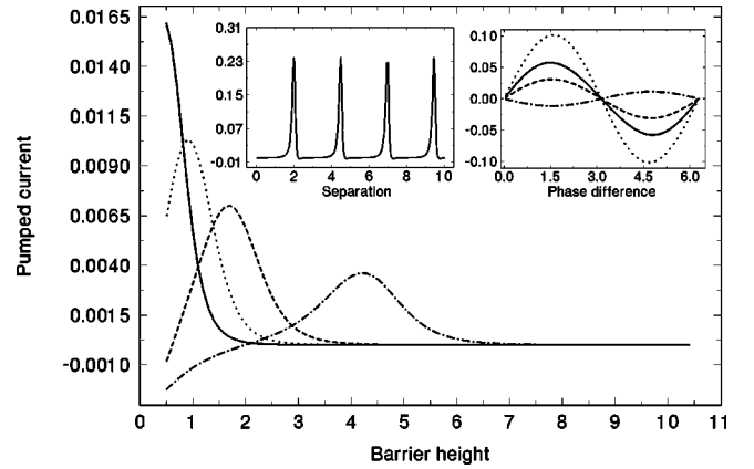
FIG. 2. The pumped current versus barrier height V_0 for different Fermi energies. Solid line: E_F = 0.45 ; dotted line: E_F = 0.75 ; dashed line: E_F = 1.1 ; dash-dotted line: E_F = 1.65 . Other parameters are a = 1, \phi = \pi/2 , and V_p = 0.4 . First inset (the left): the pumped current versus separation 2a with E_F = 1.6 and V_0 = 4 . Second inset: The pumped current versus phase difference \phi for the four different Fermi energies at V_0 = 1.0 . We have multiplied I_p in the insets by a factor of 10.
