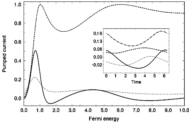
FIG. 1. The pumped current (solid line), emissivity (dotted line), and transmission coefficient (dashed line) versus Fermi energy with V_0 = 1.0 . For illustrating purpose, we have multiplied I_p by a factor of 10. Other parameters are a = 1, \phi = \pi/2 , and V_p = 0.4 . Inset: q_1, q_2, dN/dX_1 , and dN/dX_2 versus time in a cycle for E_F = 1.6 .
