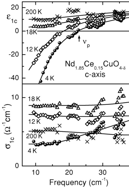
FIG. 3. Conductivity \sigma_{1c} (bottom panel) and dielectric constant \varepsilon_{1c} = -\sigma_{2c}/(\varepsilon_0\omega) (top panel) of \text{Nd}_{1.85}\text{Ce}_{0.15}\text{CuO}_{4-\delta} (sample A) along the c axis. Lines are guides to the eye. Arrow indicates the position of the c -axis plasma frequency.
