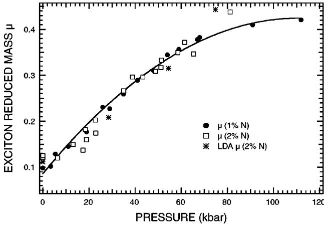
FIG. 4. Exciton reduced effective masses \mu versus pressure for 1% nitrogen (filled circles) and 2% nitrogen (open squares) samples calculated from Eq. (4) using the linewidth data shown in Fig. 3 and the \partial E_g / \partial x curve shown in Fig. 2. The smooth curve drawn through the 1% nitrogen mass data is meant to be an aid to the eye. The stars are the pressure dependent LDA calculated reduced mass.
