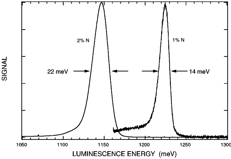
FIG. 1. Ambient pressure PL spectra at 4 K and for 1% nitrogen (right trace) and 2% nitrogen (left trace) in \text{In}_y\text{Ga}_{1-y}\text{As}_{1-x}\text{N}_x . The linewidths are \sigma(1\% \text{ nitrogen}) \approx 14 \text{ meV} and \sigma(2\% \text{ nitrogen}) \approx 22 \text{ meV} .
