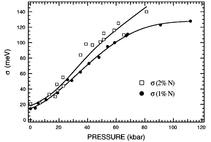
FIG. 3. The pressure dependence of \sigma for the 1% nitrogen (filled circles) and 2% nitrogen (open squares) at T = 4\text{ K} . The smooth curves drawn through the data are an aid to the eye.
