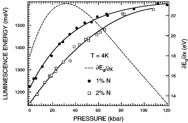
FIG. 2. The pressure dependencies of the band-gap energy for the 1% nitrogen (filled circles) and 2% nitrogen (open squares) \text{In}_y\text{Ga}_{1-y}\text{As}_{1-x}\text{N}_x samples for T = 4\text{ K} . The smooth curves drawn through the data are an aid to the eye. The right-hand axis shows the pressure variation of \partial E_g / \partial x .
