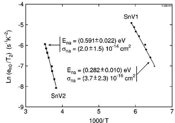
FIG. 2. Arrhenius plots of the electron emission rates for SnV1 and SnV2 of a sample from the \text{SiSn}_I crystal. The DLTS “finger prints” for this particular sample are indicated in the figure.
