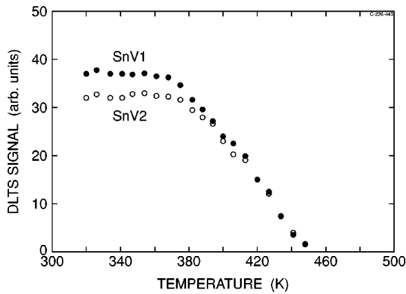
FIG. 4. Isochronal anneal sequence (30 min) of a sample from the \text{SiSn}_{III} crystal irradiated with 2-MeV electrons to a dose of 3.6 \times 10^{14} \text{ e}^-/\text{cm}^2 .
