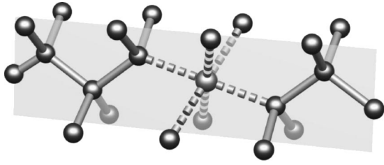
FIG. 7. Lowest-energy structure of the neutral tin split-vacancy with D_{3d} symmetry and spin-triplet ( {}^3A_{2g} ) ground state (Si-G29). The plane shown defines the (110) crystal directions. The tin impurity atom is six-fold coordinated with the Sn-Si bonds being 2.89 Å long.
