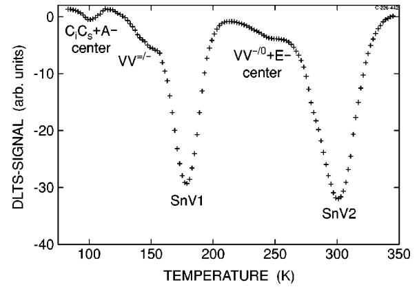
FIG. 1. DLTS spectrum of a \text{SiSn}_{II} diode immediately after a 2-MeV electron irradiation at room temperature to a dose of 2.9 \times 10^{13}\text{e}^-/\text{cm}^2 . The spectrum was recorded with a repetition rate of 250 Hz and a filling pulse width of 140\ \mu\text{s} .
