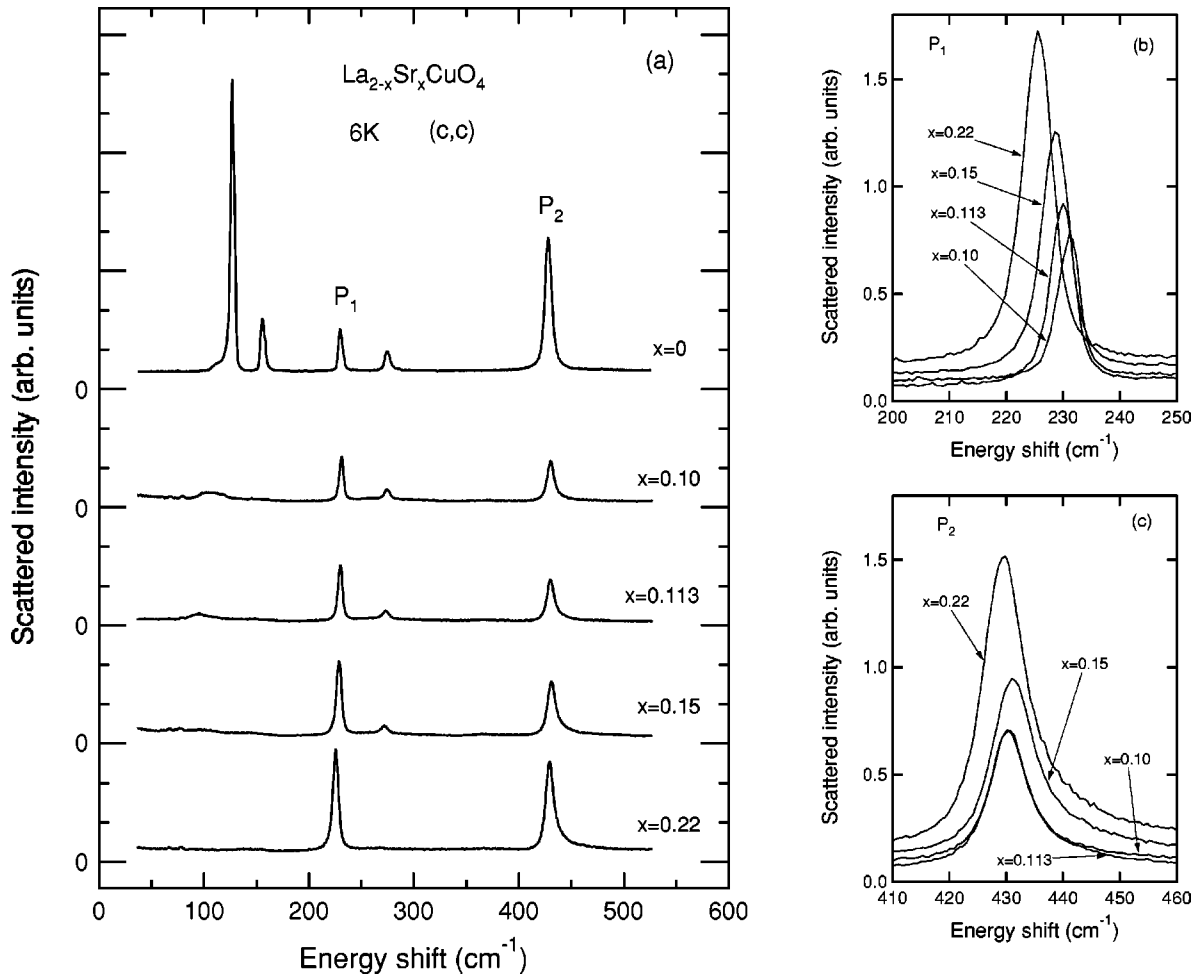
FIG. 1. (a) Sr-concentration dependence of the (c,c) Raman spectra in \text{La}_{2-x}\text{Sr}_x\text{CuO}_4 at 6 K. Each spectrum is shifted vertically to avoid the overlaps. (b) Enlarged Raman spectra around P_1 . (c) Enlarged Raman spectra around P_2 .
