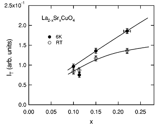
FIG. 5. x dependence of the total background intensity ( I_T ) at 6 K and room temperature. The error bar for the horizontal direction at x=0.22 is caused by a deviation from the stoichiometric oxygen concentration.
