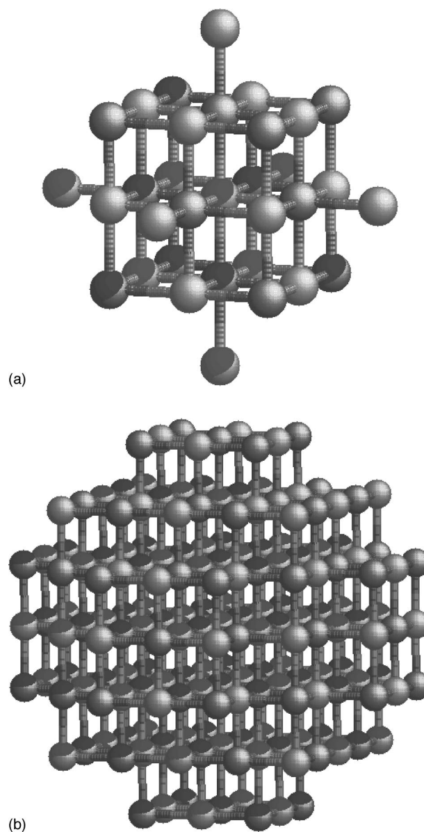
FIG. 1. The active cluster (\text{Imp}A_{92}X_{86})^{5+} employed to represent the region around the impurity, where \text{Imp} = \text{Ag}, \text{Cu} ; light spheres are cations and dark spheres anions. The core of the cluster, formed by the four first coordination shells, which are allowed to breathe, is also indicated separately.
