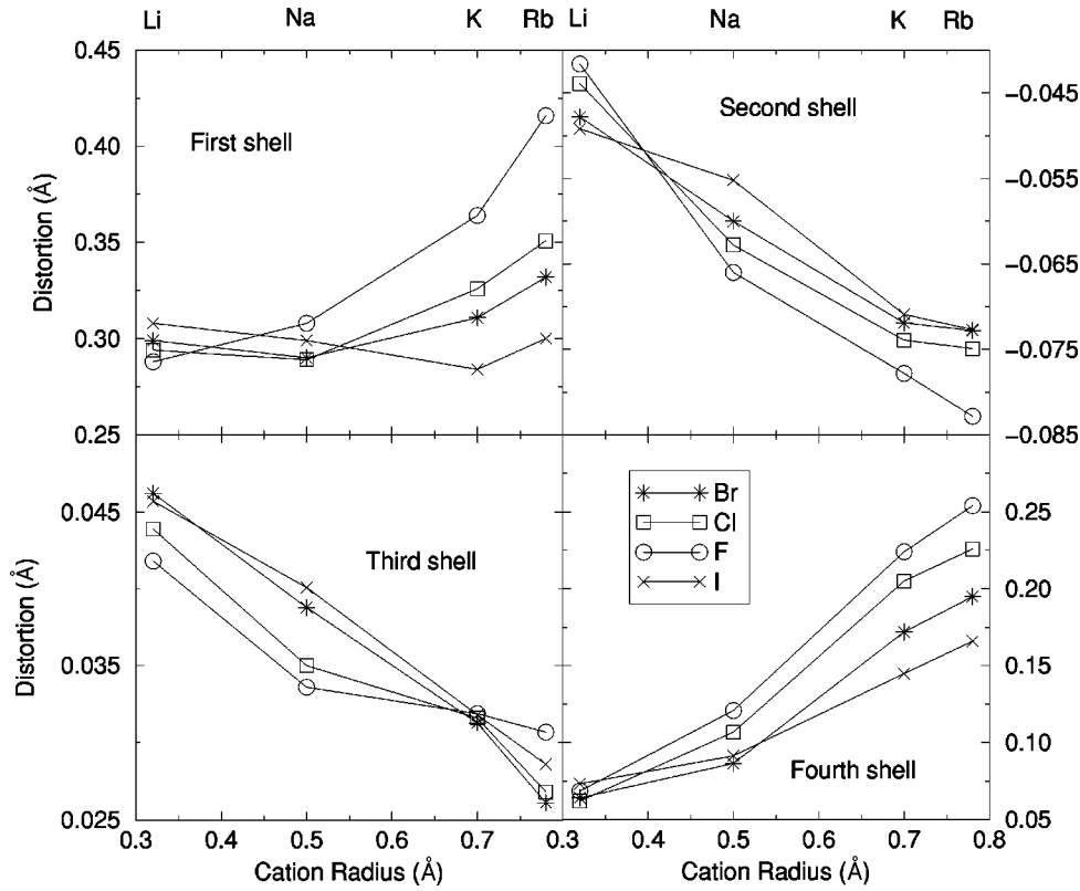
FIG. 2. Shell distortions \Delta R_i ( i=1,2,3,4 ) around \text{Ag}^- , plotted as a function of cation size.
