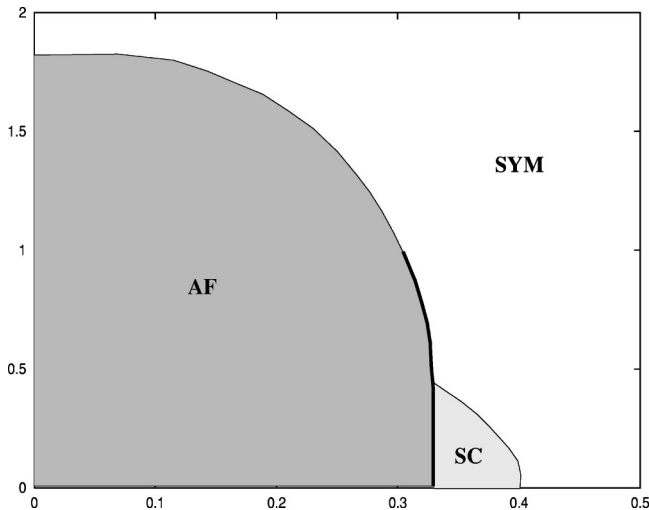
FIG. 3. The T - \rho phase diagram for h_\rho = h_\alpha = h_\delta = 2\sqrt{10U} with symmetric (SYM), antiferromagnetic (AF), and superconducting phase (SC). In the region marked by the bold line the phase transition into the antiferromagnetic phase is of first order; all other phase transitions are of second order.
