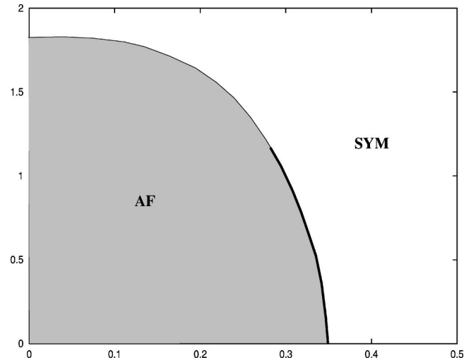
FIG. 5. The T - \rho phase diagram for h_\delta = \sqrt{10U} , h_\rho = h_\alpha = 2\sqrt{10U} with symmetric (SYM) and antiferromagnetic (AF) phase. In the region marked by the bold line the phase transition into the antiferromagnetic phase is of first order, otherwise of second order.
