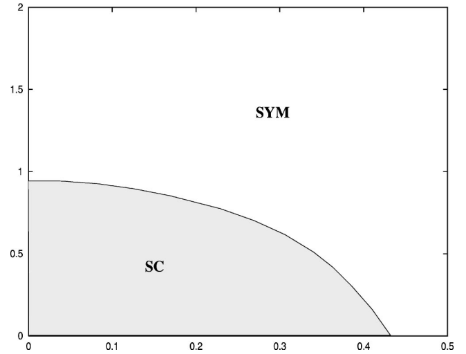
FIG. 4. The T - \rho phase diagram for h_\alpha = \sqrt{10U} , h_\rho = h_\delta = 2\sqrt{10U} with symmetric (SYM) and superconducting (SC) phase. The phase transition is of second order.
