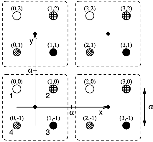
FIG. 1. The colored Hubbard model. The lattice sites of the coarse lattice are symbolized by a diamond. The numbering of the sites of our original lattice is also shown.
