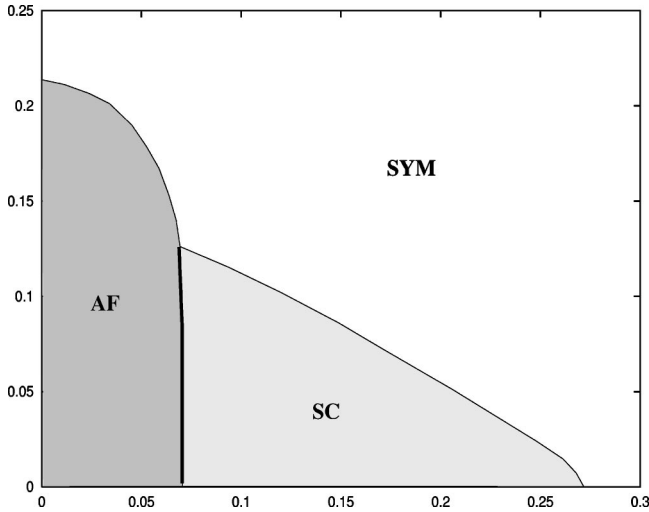
FIG. 2. The T - \rho phase diagram for h_\rho = h_\alpha = h_\delta = \sqrt{10U} with symmetric (SYM), antiferromagnetic (AF), and superconducting phase (SC). In the region marked by the bold line the phase transition into the antiferromagnetic phase is of first order; all other phase transitions are of second order.
