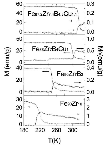
FIG. 2. FC measurements with an applied field of 100 mT (left axis) and thermoremanence curves obtained when cooling the sample down in zero-field conditions and measuring the magnetic moment on increasing the temperature (right axis).
