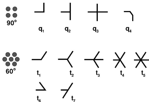
FIG. 11. Quadratic ( 90^\circ symmetry) and triangular ( 60^\circ symmetry) lattice crystals with some of the most obvious configurations of waveguide connections (branching points) for the redistribution of energy.
