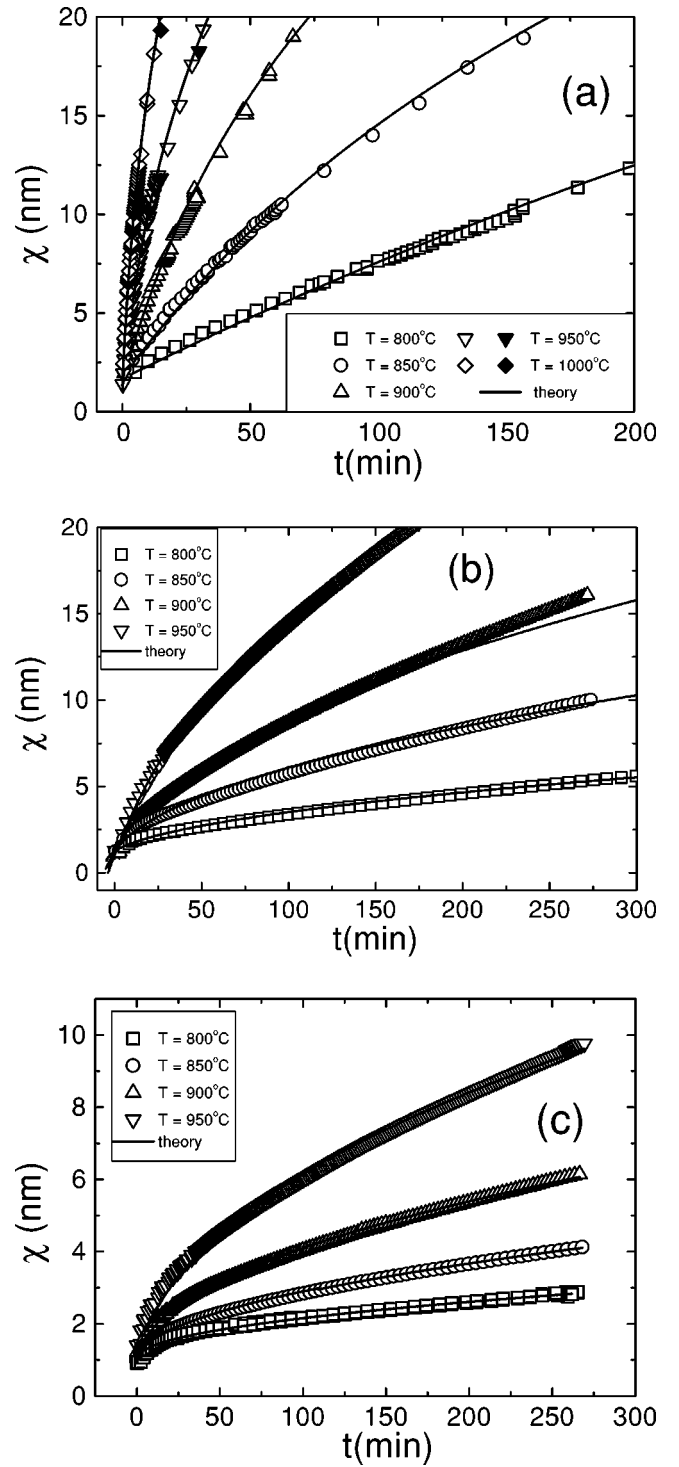
FIG. 4. Theoretical and experimental data comparison for different experiments: open symbols from Ref. 6 and solid symbols from Ref. 37. The theoretical curves were obtained by using the fitting procedure explained in the text. The oxygen partial pressure in the gas phase p_{O_2} in experiments was (a) 1 atm, (b) 0.1 atm, and (c) 0.01 atm.
