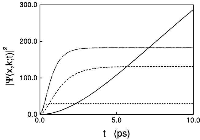
FIG. 1. This graph illustrates the building up of the probability density for the two examples discussed in the text. In the symmetrical system we show the time evolution for |\Psi(x, k; t)|^2 for incidence at \varepsilon_1=37.8 meV (solid line), \varepsilon_2=149.2 meV (dashed line), and \varepsilon_3=325.7 meV (dotted line). The fixed positions x are 80 \text{ \AA} , 48 \text{ \AA} , and 80 \text{ \AA} , respectively. In the asymmetric case \varepsilon_1=89.1 meV (dashed-dotted line) at x=55 \text{ \AA} .
