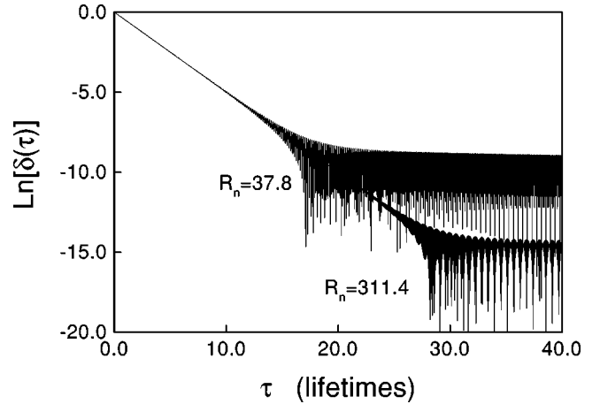
FIG. 3. Exponential and nonexponential contributions to the buildup. We plot the logarithm of the difference of \delta(\tau) = |1 - |\Psi(\tau)/\phi|| versus \tau , for the states n=1 and n=3 of the symmetrical system considered in the text. The corresponding values of the ratios R_n \equiv \epsilon_n/\Gamma_n are shown in the figure. The linear behavior corresponds to the exponential regime, and the deviations from it appear after a certain transition time \tau_{\text{onset}} .
