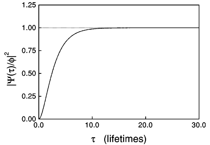
FIG. 2. Evolution of |\Psi(\tau)/\phi|^2 as a function of \tau for the same cases of Fig. 1. All four curves become identical. For comparison, a plot of |\Psi(\tau)/\phi|^2 using Eq. (6) is also included. The resulting values are also superimposed on the other curves illustrating that they obey a simple exponential law with a unique transient time constant of two lifetimes.
