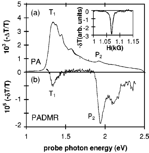
FIG. 4. PA spectrum (a) compared to \lambda -PADMR spectrum (b) of spin-1/2 excitations, measured at H=1065 G ( g=2 ) and 10 K. The inset shows the H-PADMR spectrum at 1.9 eV.
