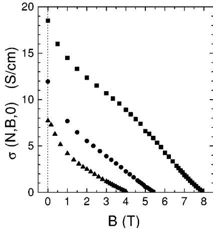
FIG. 3. Zero-temperature conductivity \sigma(N, B, 0) of Samples A3, B2, and B4 vs magnetic induction B .
