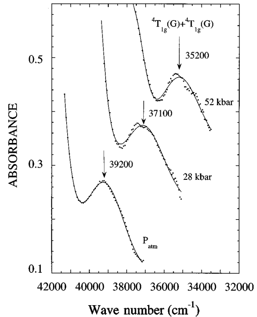
FIG. 3. Variation of the uv band at 39200 \text{ cm}^{-1} in \text{NH}_4\text{MnCl}_3 with pressure at room temperature. The spectra have been fitted to the sum of an absorption background plus a single Gaussian which are shown (full lines) together with the absorption data (points). Arrows indicate the maximum position of the fitted Gaussian band. Note the important redshift experienced by this band ( -76 \text{ cm}^{-1}/\text{kbar} ) in comparison to the single excitation shifts shown in Fig. 2. The spectra are displaced for comparison purposes.
