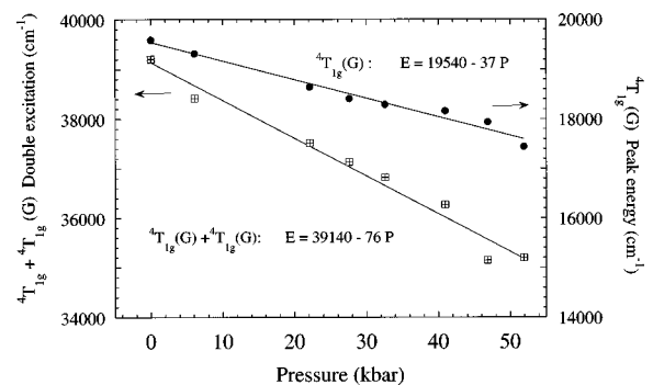
FIG. 4. Variation of the peak energy of the uv band at 39200 \text{ cm}^{-1} and the first {}^4T_{1g} band at 19590 \text{ cm}^{-1} with pressure in the 0–60 kbar range. Straight lines represent the least-square linear fits of the experimental data. Note that the shift rate of the uv band is almost exactly twice the shift rate of the {}^4T_{1g}(G) single excitation band.
