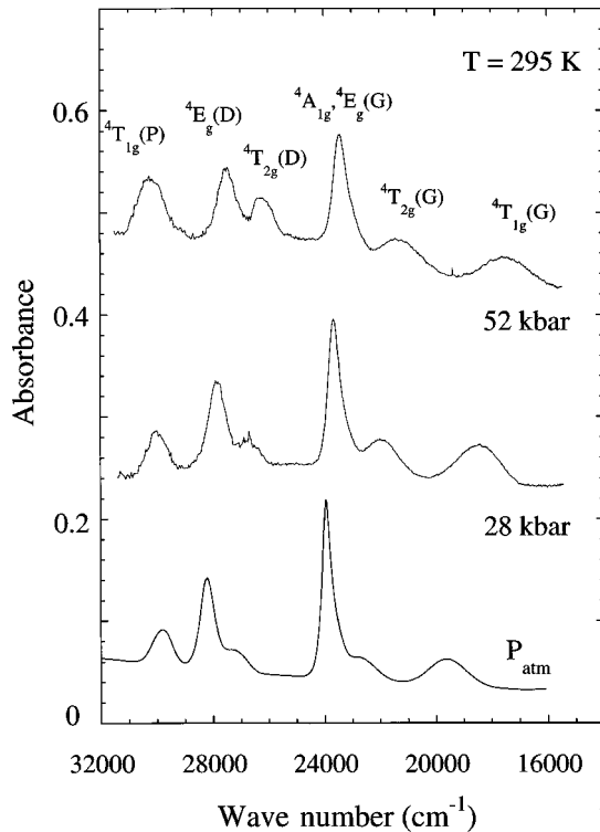
FIG. 2. Variation of the optical-absorption spectrum of the \text{NH}_4\text{MnCl}_3 microcrystal with pressure at T=295 K. Note the different shifts undergone by the {}^4T_{1g}(G) and {}^4A_{1g}{}^4E_g(G) bands. The spectra are displaced for comparison purposes.
