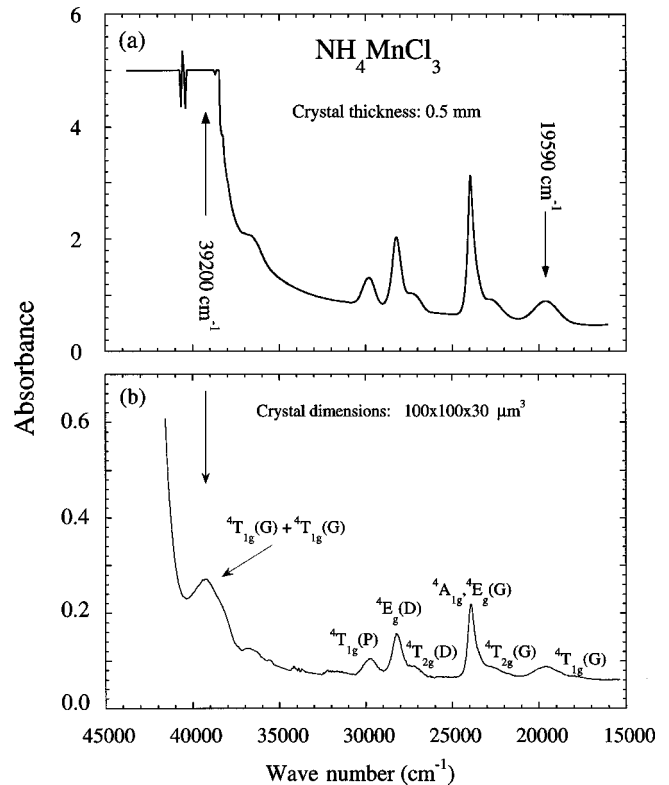
FIG. 1. (a) Optical-absorption spectrum of the \text{NH}_4\text{MnCl}_3 perovskite at ambient pressure and room temperature recorded with a conventional spectrometer. Crystal dimensions: 3 \times 3 \times 0.5\text{ mm}^3 . The horizontal line in the uv region indicates the detection limit of the instrument. (b) Optical-absorption spectrum of a \text{NH}_4\text{MnCl}_3 microcrystal ( 100 \times 100 \times 30\text{ }\mu\text{m}^3 ) obtained with the experimental setup described elsewhere (Refs. 19 and 20). Bands are identified with the commonly used labels (Refs. 17 and 21). Although the energy of the \text{Mn}^{2+} single excitation bands are the same in (a) and (b), note the presence of an intense band at 39\,200\text{ cm}^{-1} in (b).
