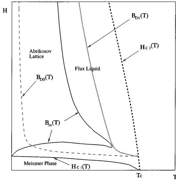
FIG. 3. A sketch (not to scale) of the phase diagram showing the location of the “disentanglement” lines for the liquid discussed in the text. The dashed line, B_{D0}(T) , marks the breaking down of the perturbation expansion for the inverse tilt modulus; the dotted line, B_{D1}(T) , corresponds to n_n/n_0=1 and signals the divergence of the conjectured form of c_{44}^R , given in Eq. (7.18). The width of the reentrant liquid phase is in reality much smaller than shown here and the line B_{D0}(T) may or may not pass through it. B_m(T) is the melting line. H_{c2}(T) marks the onset of a Meissner effect and is not a sharp phase transition. Notice that the part of B_{D0}(T) which lies within the lattice phase is not meant to represent any real transition or crossover whatsoever.
