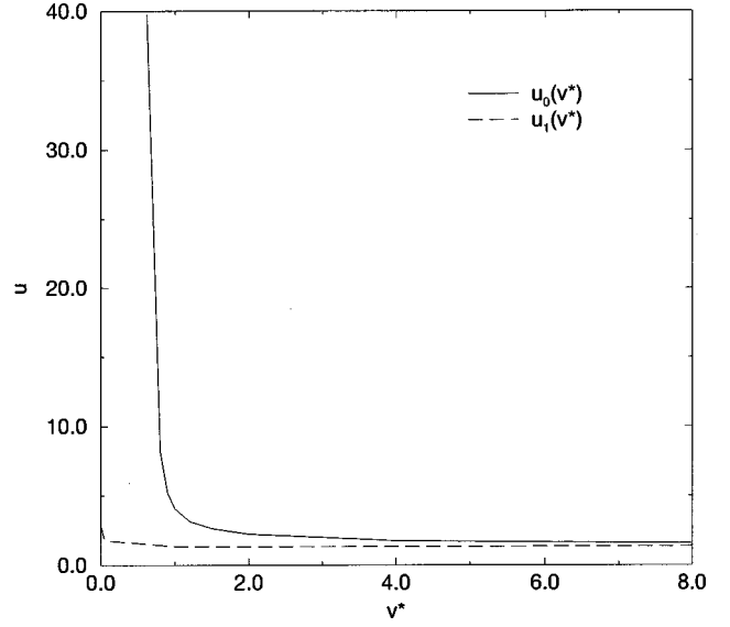
FIG. 2. The solid line is the numerical solution of Eq. (7.17). It defines the line u_0(v^*) in the (u, v^*) parameter space where the perturbation expansion of the tilt autocorrelator breaks down. The dashed line is u_1(v^*) , where n_n/n_0 = 1 .
