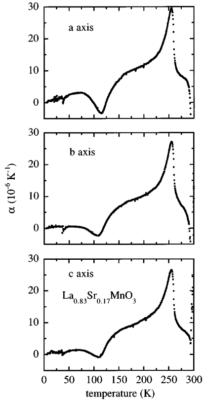
FIG. 4. Thermal-expansion coefficient \alpha vs temperature for the three orthorhombic axes. Data are shown for temperatures below the structural transition.
