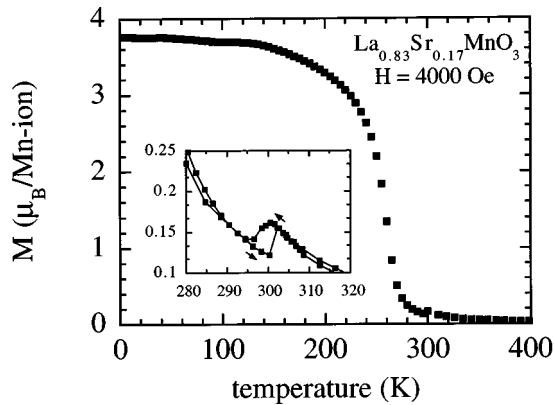
FIG. 1. Magnetization vs temperature at 4000 Oe. In the inset, the region near 300 K is enlarged; the arrows indicate cooling and warming.
