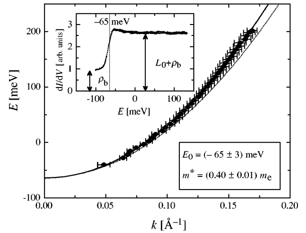
FIG. 4. Dispersion relation of the Ag(111) surface state. The solid line is a quadratic fit to our STM data and the dotted line shows results from photoemission data at 65 K (Ref. 3). The inset shows dI/dV data taken on a perfect terrace ( V=497 mV, I=5.0 nA). The contribution of the surface LDOS to the measured total LDOS is L_0/(\rho_{\text{bulk}}+L_0)\approx 0.64 .
