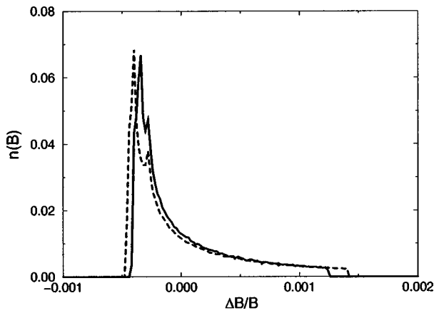
FIG. 5. Solid line: Magnetic-field distribution obtained from the nonlinear-nonlocal London equation. Dashed line: Magnetic-field distribution obtained from a London equation including only the additional nonlocal term using the same parameters.
