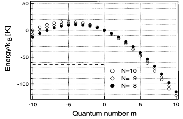
FIG. 10. Position of the energy levels at three different values of the magnetic field, corresponding to resonances N=8, 9 , and 10 , respectively. The dashed line is the energy of the m = \pm 10 levels at zero field, corresponding to the zero-field barrier height. The barrier for magnetization reversal is significantly reduced with these magnetic fields while the energy gained when a state near the top of the barrier decays to the stable m = 10 state is growing.
