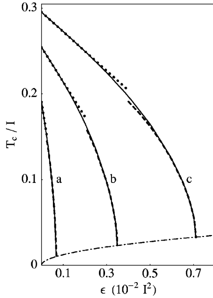
FIG. 3. The critical temperature T_c(\epsilon) of the anisotropic RFIM as a function of the random magnetic-field strength for \tilde{I}_\perp/I = 0.002, 0.01, \text{ and } 0.02 (curves a, b, and c, respectively). Solid curves derive from solving Eq. (11) with the exact free energy Eq. (40). The dashed curves are obtained by solving Eq. (61), while the dots represent the small- \epsilon behavior Eq. (49). The dash-dotted curve shows the temperature T_0(\epsilon) , below which the continuum approximation breaks down and which corresponds approximately to T = 0 in the discrete RFIM.
